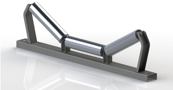
STAZIONI PER TERNE A 30° 30° STATION FOR BACKHOE LOADERS
