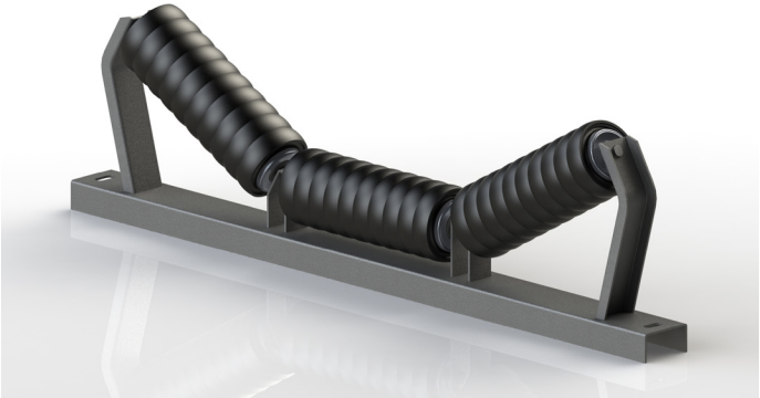
STAZIONI PER TERNE A 30° CON RULLI D'IMPATTO 30° STATION FOR BACKHOE LOADERS WITH IMPACT ROLLERS
